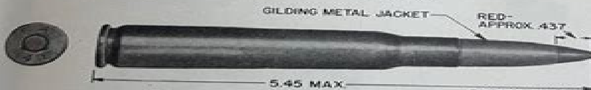
FIGURE 8.—Cartridge, tracer, caliber .50.
