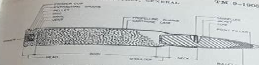
FIGURE 5.—Section of ball cartridge, caliber .50.
