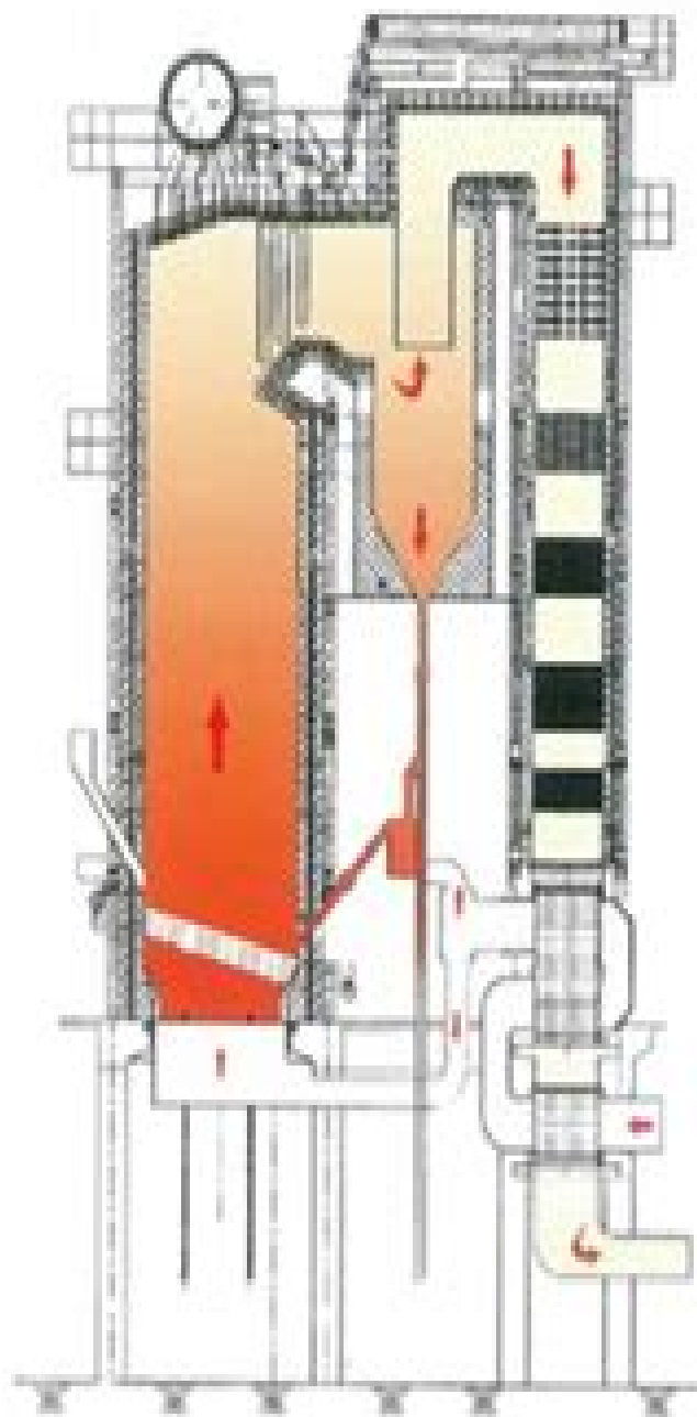
General Plan of Low-speed Bed CFB
