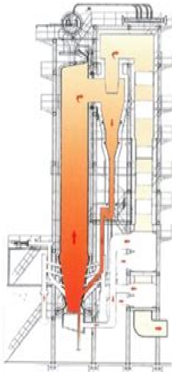
General Plan of Medium-speed Bed CFB
