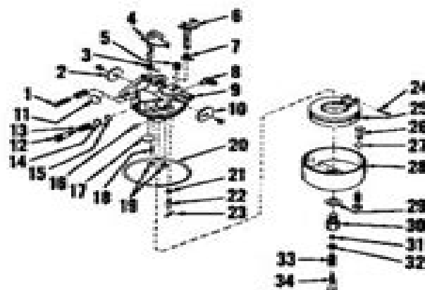
Fig. 71—Exploded view of Tecumseh carburetor.
