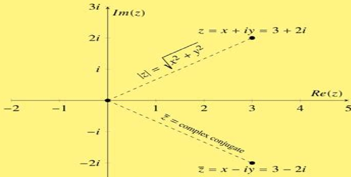
Figure 1.1: The Complex Plane
