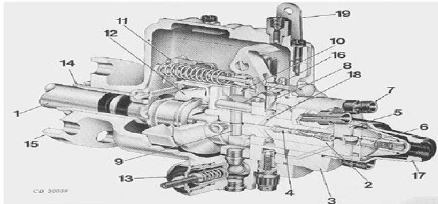
Stanadyne Fuel Injection Pump (DB2/DB4)
