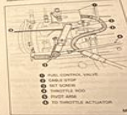
Throttle Actuator Lever Bracket — Pivot Arm Configuration
