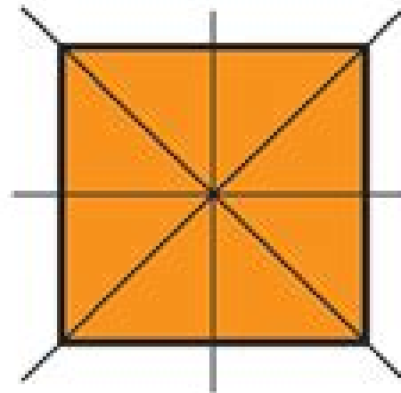
D4 - Symmetry about four axis
