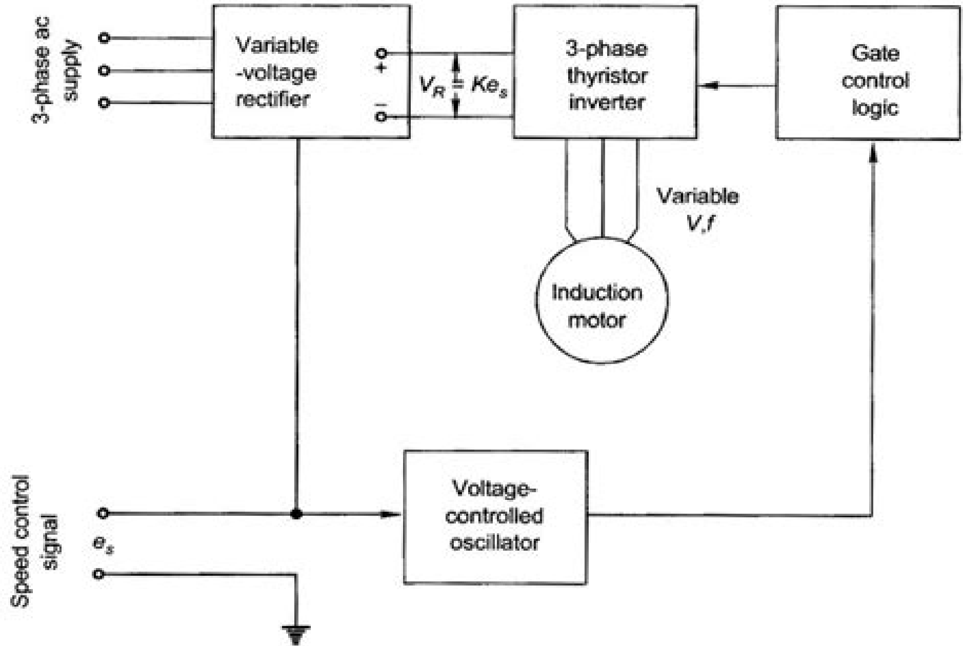
Fig. 11.38 Frequency-control of induction motor speed; \text{speed} \propto e_s , flux/pole constant
