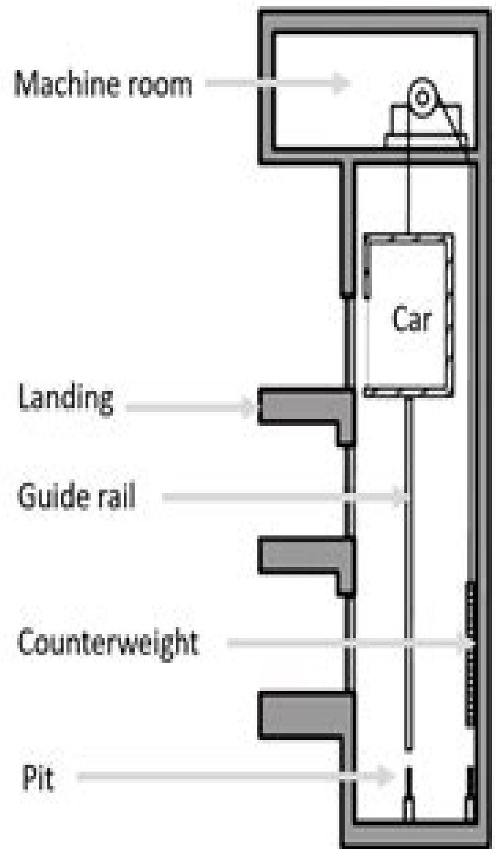
Traction Elevators
