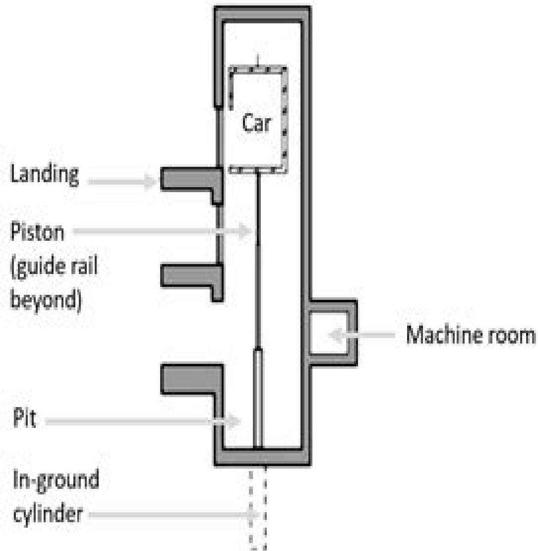
Hydraulic Elevators
