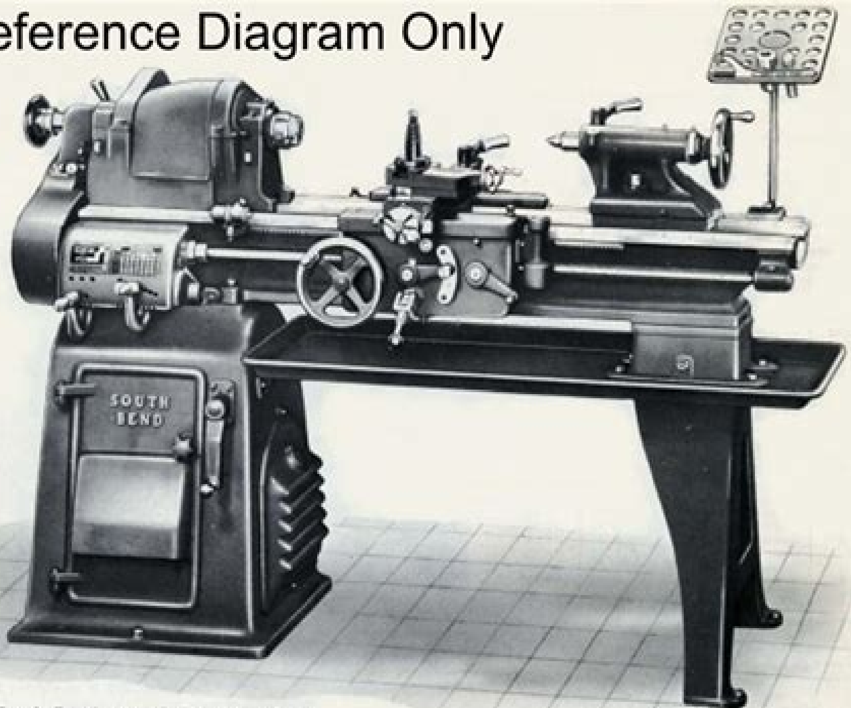
The South Bend 13-inch Precision Lathe
