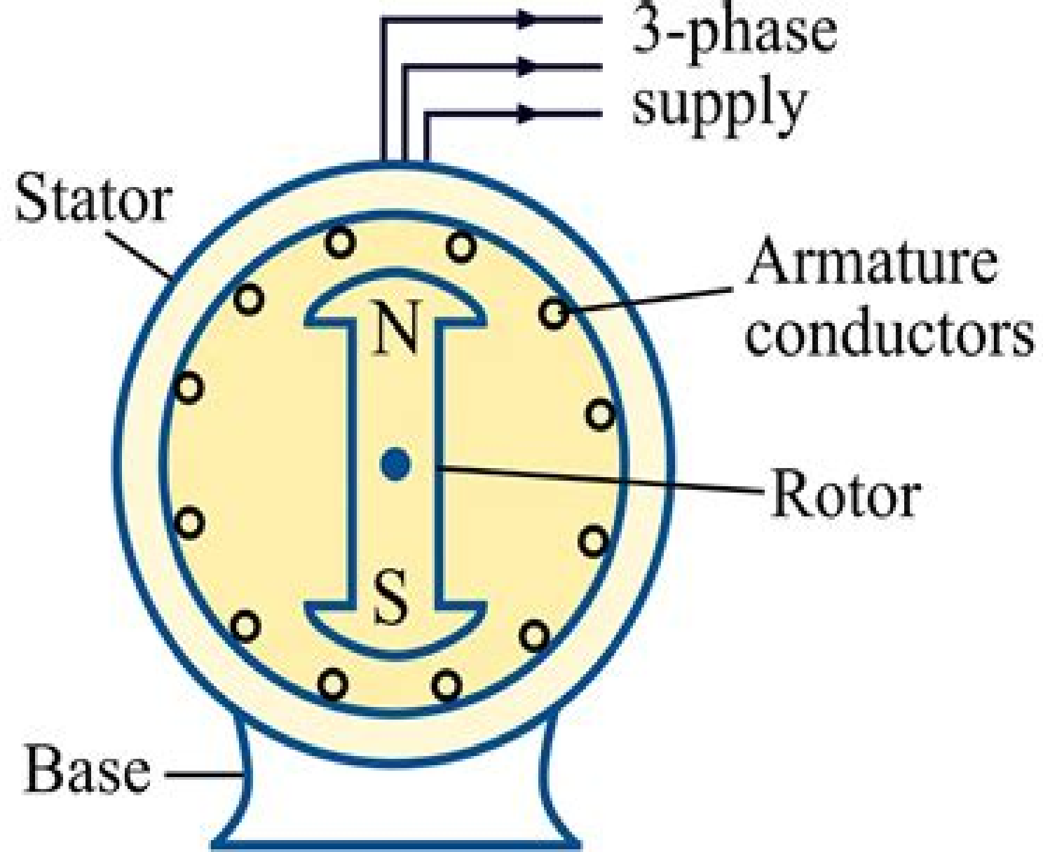
Figure 1 - Synchronous Generator
