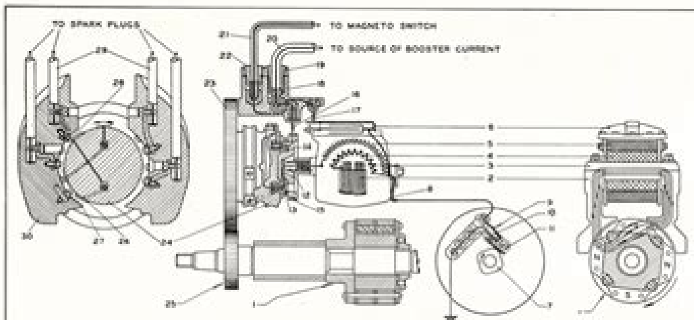
SCHEMATIC DIAGRAM OF ELECTRIC AND MAGNETIC CIRCUITS
