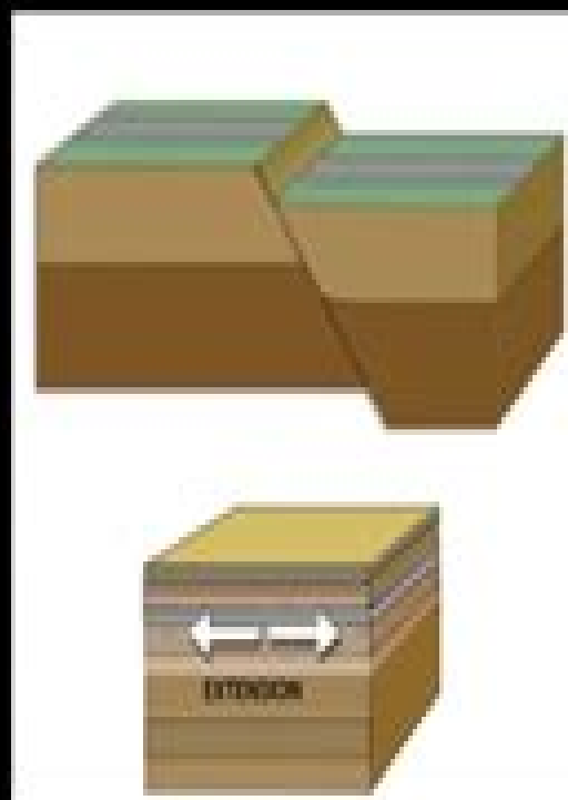
Normal fault
