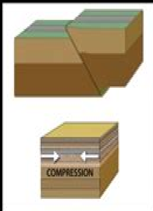
Reverse fault
