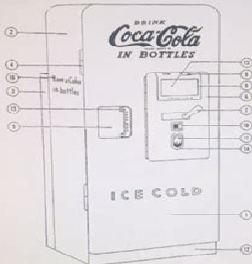
Figure 10-32, Cavalier, Model CM-31V, Cooler Exterior
