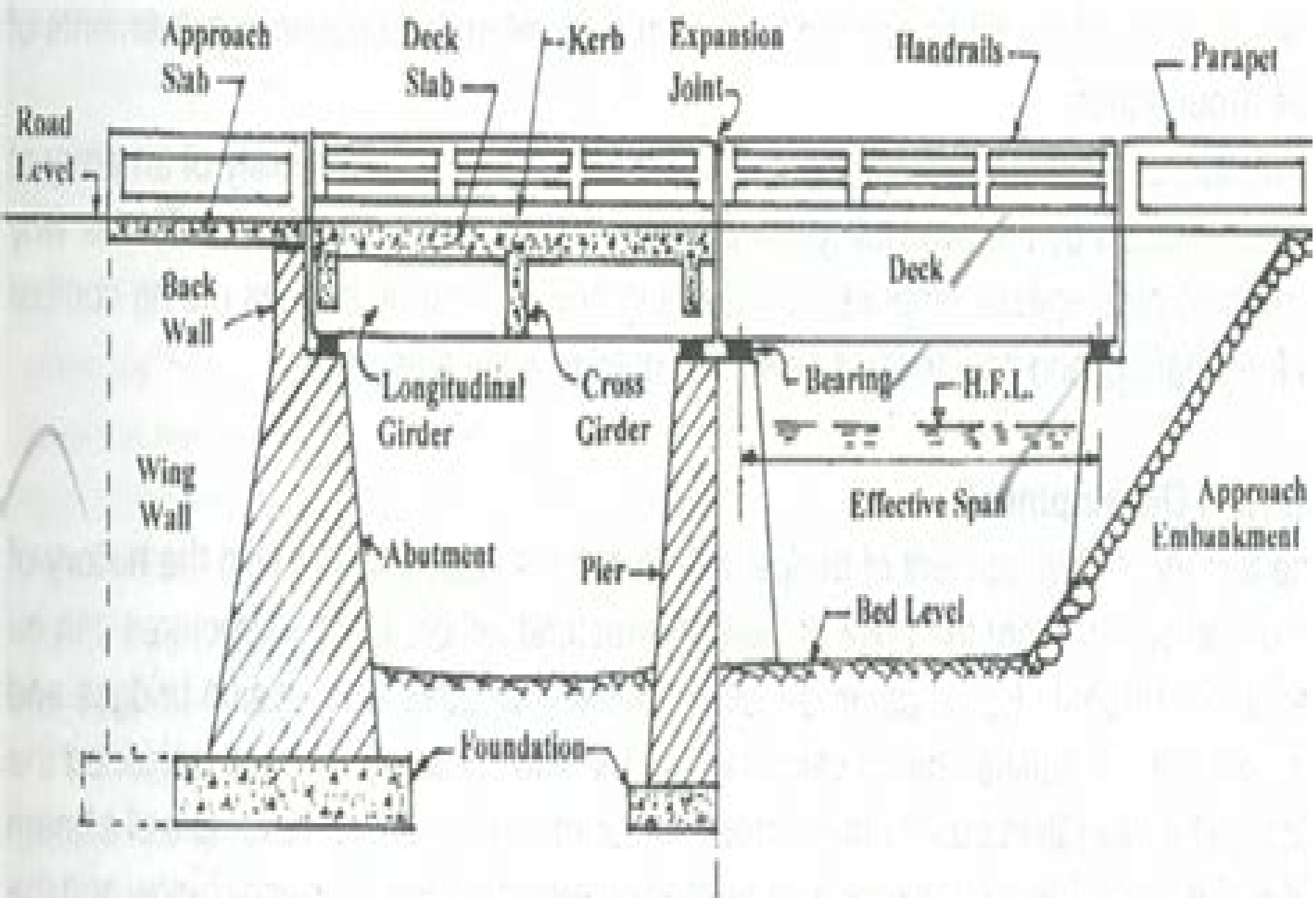
Figure 1.1 Components of a Typical Bridge.
