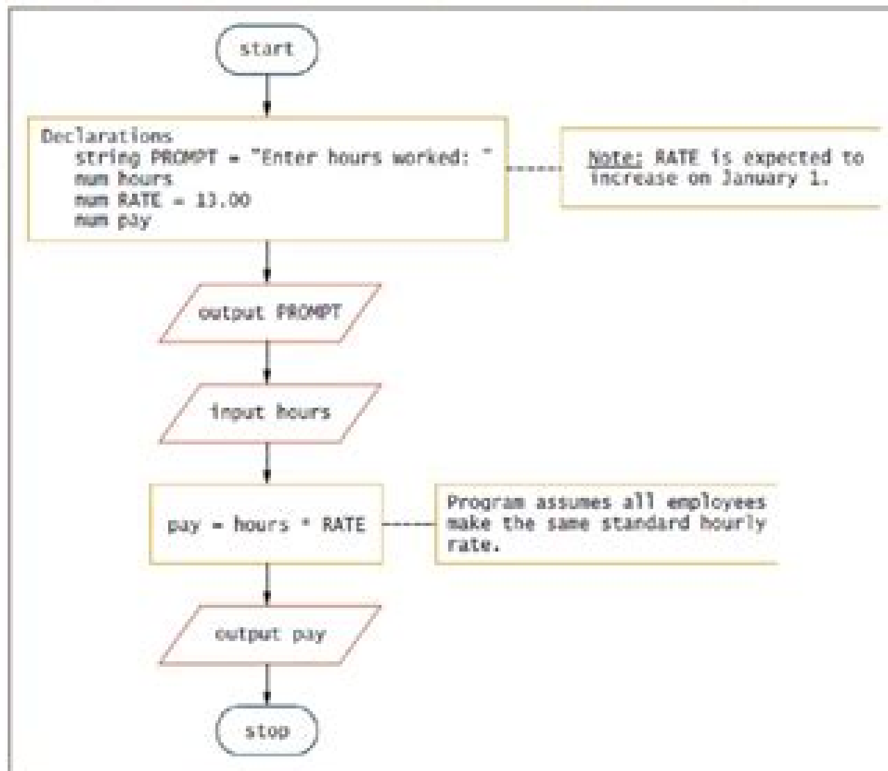
Figure 2-13 Flowchart that includes annotation symbols
