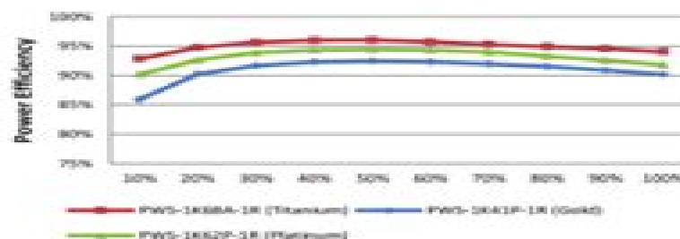
Figure 2 - Power Efficiency for Gold/Platinum/Titanium Level PSU.
