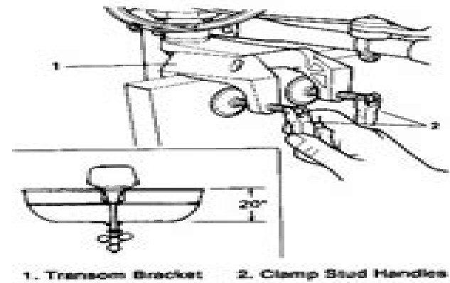
Figure 5: Mounting to Transom
