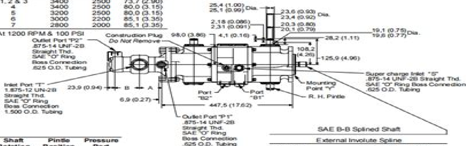
Cover-End Vane Pump
