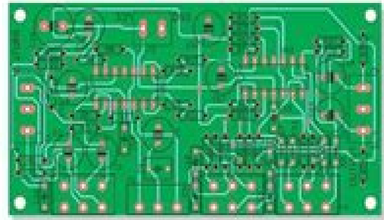
PCB Layout
